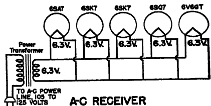
A-C RECEIVER
